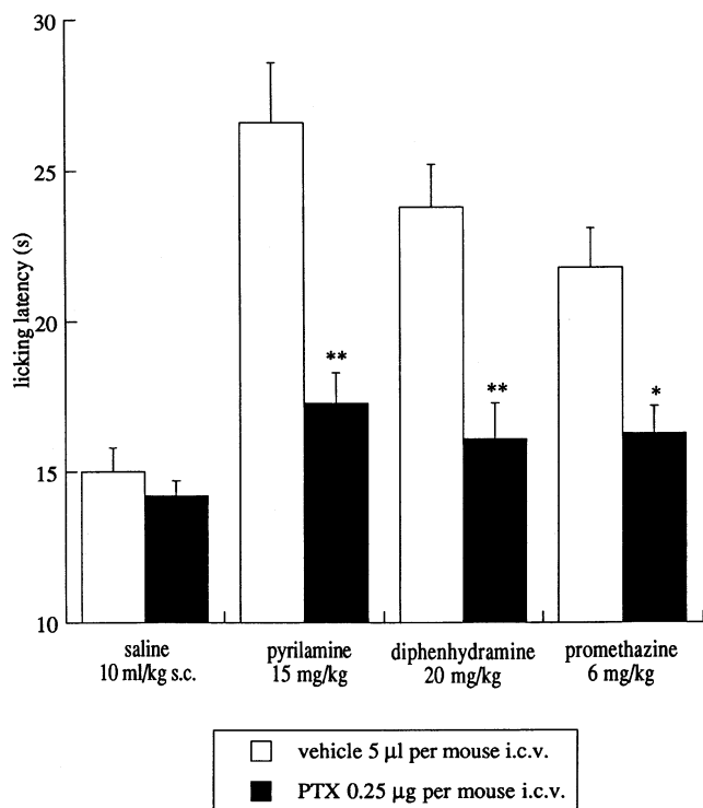
Fig. 2. Prevention by pertussis toxin (PTX) pretreatment of antinociception induced by pyrilamine (15 mg/kg s.c.), diphenhydramine (20 mg/kg s.c.) and promethazine (6 mg/kg s.c.) in the mouse hot-plate test. The test was performed 7 days after a single i.c.v. injection of vehicle or PTX (0.25 µg/mouse i.c.v.). Vertical lines represent SEM; between 14 and 18 mice were tested. * P < 0.05 , ** P < 0.01 in comparison with corresponding analgesic-treated mice.
