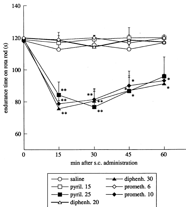
Fig. 7. Effect of pyrilamine (15–25 mg/kg s.c.), diphenhydramine (20–30 mg/kg s.c.) and promethazine (6–10 mg/kg s.c.) in the mouse rota rod test. Vertical lines give SEM; there were 10 mice/group. * P < 0.05 , ** P < 0.01 in comparison with saline-treated mice.
