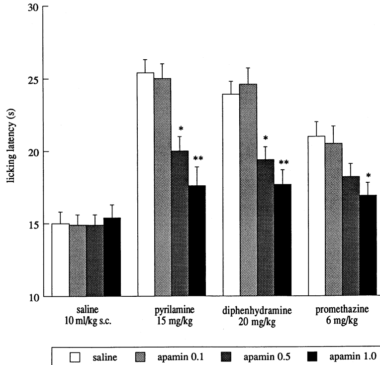
Fig. 5. Prevention by the Ca^{2+} -gated K^+ channel blocker apamin (0.1–1.0 ng/mouse i.c.v.) of pyrilamine (15 mg/kg s.c.), diphenhydramine (20 mg/kg s.c.) and promethazine (6 mg/kg s.c.) antinociception in the mouse hot-plate test. Vertical lines give SEM; there were 15 mice/group. * P < 0.05 , ** P < 0.01 in comparison with saline-treated mice.
