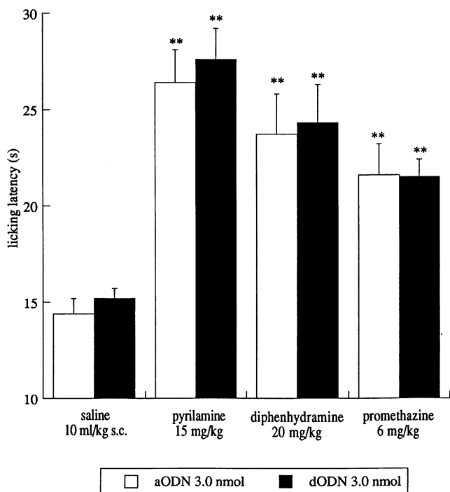
Fig. 6. Lack of effect of an antisense ODN (aODN) to the mKv1.1 gene on pyrilamine- (15 mg/kg s.c.), diphenhydramine- (20 mg/kg s.c.) and promethazine- (6 mg/kg s.c.) induced antinociception in the mouse hot plate test. Mice were injected with antisense ODN (aODN) or degenerated ODN (dODN) at the dose of 3.0 nmol/single i.c.v. injection on days 1, 4 and 7. The test was performed 72 h after the last i.c.v. injection of degenerate dODN or aODN. Vertical lines give SEM; there were 15–18 mice/group. ** P < 0.01 in comparison with saline-treated mice.
