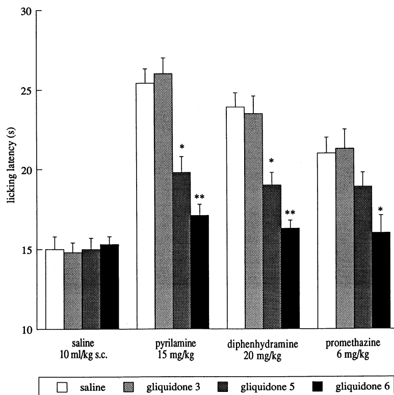
Fig. 3. Prevention by the K_{ATP} blocker gliquidone (3.0–6.0 \mu g/mouse i.c.v.) of pyrilamine (15 mg/kg s.c.), diphenhydramine (20 mg/kg s.c.) and promethazine (6 mg/kg s.c.) antinociception in the mouse hot-plate test. Vertical lines represent SEM; between 10 and 15 mice were tested. * P < 0.05 , ** P < 0.01 in comparison with the corresponding analgesic-treated mice.
