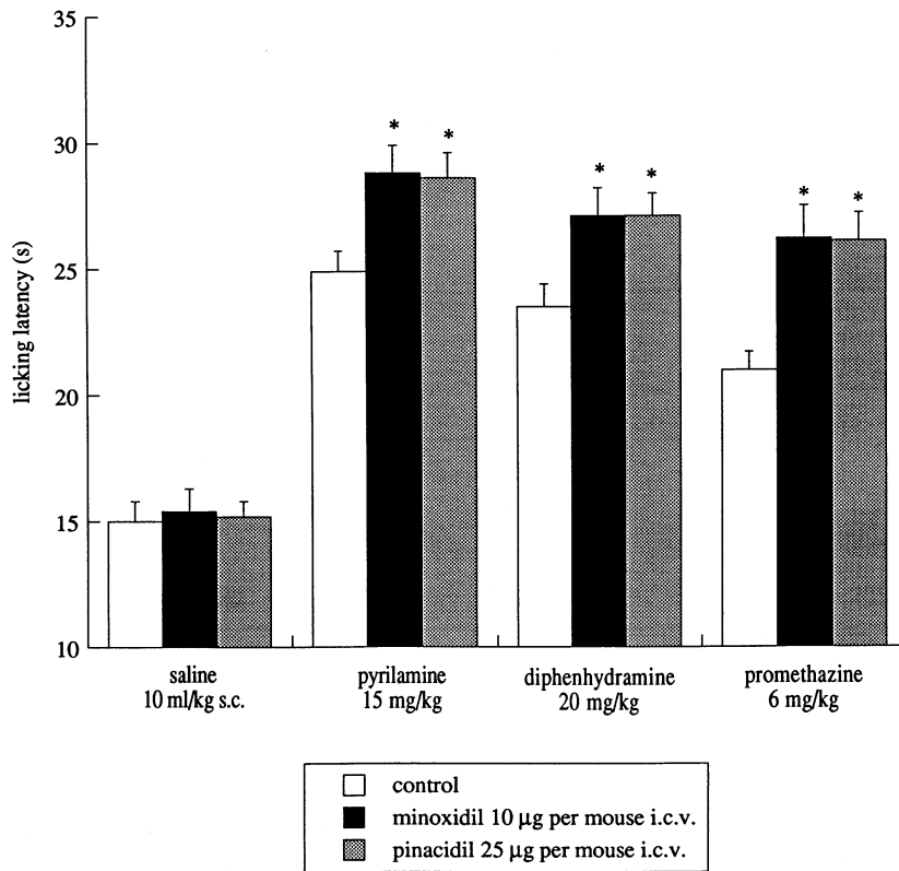
Fig. 4. Enhancement of pyrilamine (15 mg/kg s.c.), diphenhydramine (20 mg/kg s.c.) and promethazine (6 mg/kg s.c.) antinociception by the K_{ATP} openers minoxidil (10 µg/mouse i.c.v.) and pinacidil (25 µg/mouse i.c.v.) in the mouse hot plate test. Vertical lines represent SEM; between 14 and 19 mice were tested. * P < 0.05 in comparison with corresponding analgesic-treated mice.
