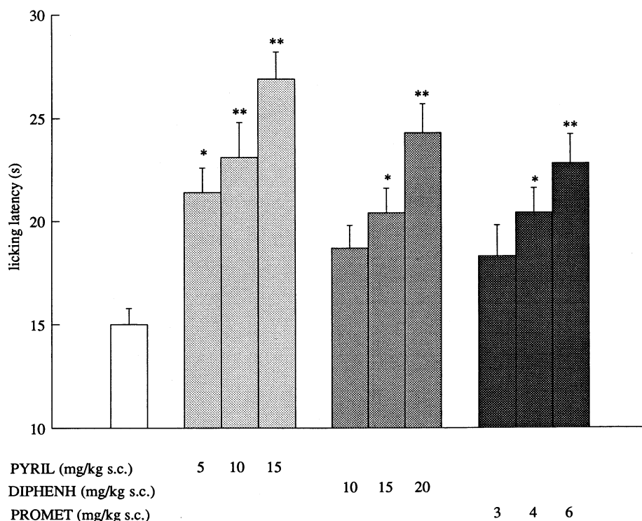
Fig. 1. Dose-response curve of pyrilamine (5–15 mg/kg s.c.), diphenhydramine (10–20 mg/kg s.c.) and promethazine (3–6 mg/kg s.c.) in the mouse hot-plate test. Vertical lines represent SEM; between 10 and 14 mice were tested. * P < 0.05 , ** P < 0.01 in comparison with saline-treated mice.
