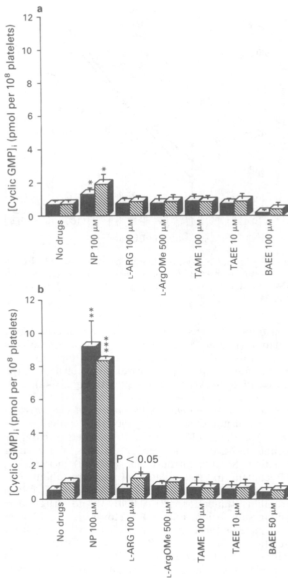
Figure 4 (a) Effect of L-arginine esters (tested at concentrations near their IC_{50} values for inhibition of \alpha -thrombin-induced [Ca^{2+}]_i increase) in comparison with 100 \mu M sodium nitroprusside (NP) and 100 \mu M L-arginine on cyclic GMP concentration measured in human platelets suspended in HEPES/NaHCO 3 buffer containing 1 mM CaCl 2 , 10 \mu M indomethacin, 100 u ml^{-1} apyrase and 30 \mu M isobutyl methyl xanthine (IBMX), estimated either at rest (solid columns) or after stimulation by \alpha -thrombin (0.03 u ml^{-1} ) (hatched columns). Values are the mean ( \pm s.e.mean) of at least 3 experiments. * P < 0.05 vs no drugs. (b) Effect of L-arginine esters (tested at concentrations near their IC_{50} values for inhibition of \alpha -thrombin-induced [Ca^{2+}]_i increase) in comparison with 100 \mu M sodium nitroprusside (NP) and 100 \mu M L-arginine on cyclic GMP concentration measured in human platelets suspended in HEPES/NaHCO 3 buffer containing 1 mM CaCl 2 and 30 \mu M isobutyl methyl xanthine (IBMX), estimated either at rest (solid columns) or after stimulation by \alpha -thrombin (0.03 u ml^{-1} ) (hatched columns). Values are the mean ( \pm s.e.mean) of at least 3 experiments. ** P < 0.001 vs no drugs; *** P < 0.0001 vs no drugs.
