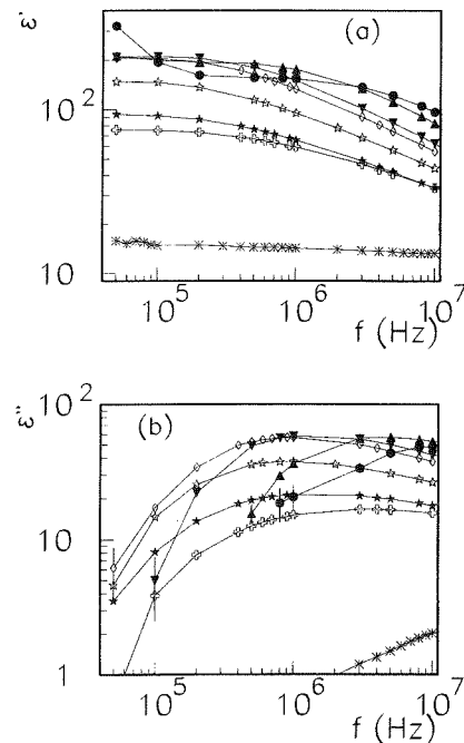
FIG. 6. \epsilon'(f) and \epsilon''(f) experimental values [(a) and (b), respectively], at T=20^\circ\text{C} , for the samples with \phi : 0.600 (full points), 0.515 (full triangles), 0.429 (full reversed triangles), 0.408 (open diamond), 0.361 (open stars), 0.346 (full stars), 0.327 (open crosses), and 0.205 (asterisks). The increase of \epsilon' below 10^5 Hz at \phi=0.600 is due to electrode polarization. The lines are guides for the eyes.
