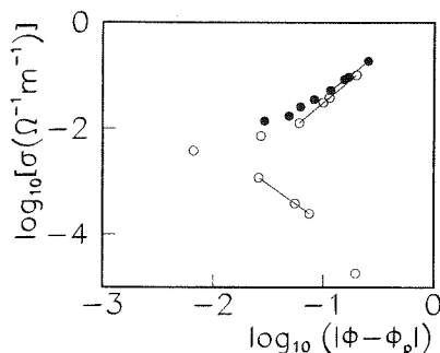
FIG. 4. Experimental values of Fig. 3 arranged to show the linear trend of the \log_{10}(\sigma) vs \log_{10}|\phi - \phi_p| below (bottom curve) and above (upper curves) the percolation threshold. The straight lines represent the fitting results. The symbol meanings are as in Fig. 3.
