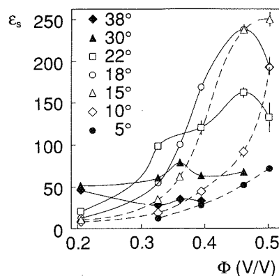
FIG. 1. Experimental \epsilon_s(\phi) values at different temperatures. Dashed lines at 5, 10, and 15 °C. Continuous lines at 18, 22, 30, and 38 °C. The lines are guides for the eyes.
