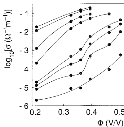
FIG. 2. Experimental \sigma(\phi) values at different temperatures. From bottom to top in the picture: T=10, 15, 18, 20, 28, 32, 38, and 40 °C. The curves show the crossing of \phi_p threshold (sigmoidal shape curve) at 15, 18, and 20 °C, the trend above \phi_p at higher temperatures (upper part of the sigmoidal shape curve) and the trend below \phi_p at the lowest temperature. The lines are guides for the eyes.
