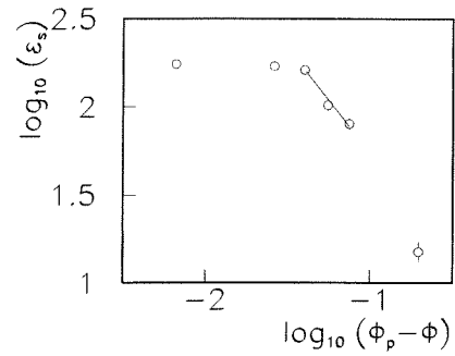
FIG. 5. Experimental values of Fig. 1 at 20^\circ\text{C} showing the linear trend \log_{10}(\epsilon'_s) vs \log_{10}(\phi_p - \phi) , below the percolation threshold.
