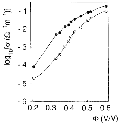
FIG. 3. Experimental \sigma(\phi) values at T=20^\circ\text{C} (open points) and T=25^\circ\text{C} (full points). The lines are guides for the eyes.
