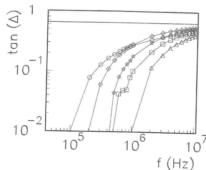
FIG. 10. Loss angle tangent vs frequency for the sample with \phi=0.205 , at temperatures 30^\circ\text{C} (points), 34^\circ\text{C} (crosses), 36^\circ\text{C} (stars), 38^\circ\text{C} (squares), and 40^\circ\text{C} (triangles). The line is \tan\Delta=0.65 .
