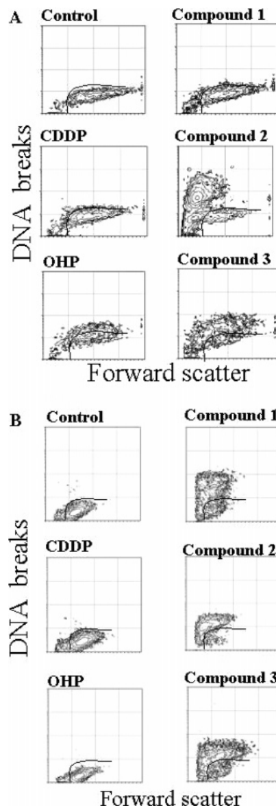
Figure 3. Apoptosis analysis. Bivariate histograms, relative to A2780/S (panel A) and A2780/R (panel B) cells, are shown for control cells and cells treated with IC 70 drug concentrations for 4 h followed by a 20 h postincubation in drug-free medium. Apoptotic breakage data (by TUNEL assay) are plotted against forward scatter.
