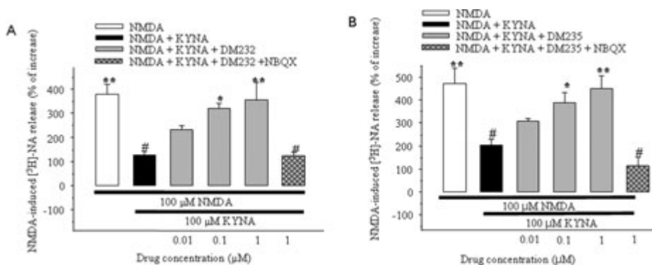
Fig. 4. Panel A: Effects of DM232 (unifiram), alone or in the presence of NBQX, in the kynurenate test. Rat hippocampal slices were labelled with [ 3 H]NE and superfused with Mg 2+ -free medium. Unifiram was added together with kynurenic acid (KYNA) and tritium release was then provoked by NMDA. In some experiments NBQX was added concomitantly with KYNA. Empty bars: 100 μM NMDA; solid bars: NMDA + 100 μM KYNA; gray bars: NMDA + KYNA + DM232 (concentration as indicated); cross hatched bars: NMDA + KYNA + 1 μM DM232 + 5 μM NBQX. Data are means ± S.E.M. of 5–7 experiments run in triplicate (three superfusion chambers for each condition). # P < 0.01 vs. NMDA; * P < 0.05 vs. NMDA + KYNA; ** P < 0.01 vs. NMDA + KYNA. Panel B: Effects of DM235 (sunifiram), alone or in presence of NBQX, in the kynurenate test. Slices were superfused with Mg 2+ -free medium from t = 0 min of superfusion. In some experiments NBQX was added concomitantly with KYNA, at t = 30 min till the end of superfusion. Empty bars: 100 μM NMDA; solid bars: NMDA + 100 μM KYNA; gray bars: NMDA + KYNA + DM235 (concentration as indicated); cross hatched bars: NMDA + KYNA + 1 μM DM235 + 5 μM NBQX. Data are means ± S.E.M. of 4–7 experiments run in triplicate (three superfusion chambers for each condition). # P < 0.01 vs. NMDA; * P < 0.05 vs. NMDA + KYNA; ** P < 0.01 vs. NMDA + KYNA. Reproduced from ref. 11 with kind permission of Springer Science and Business Media.
