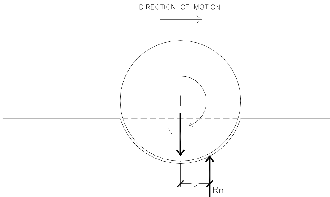
Figure 8: schematisation of the wheel/ground interaction
