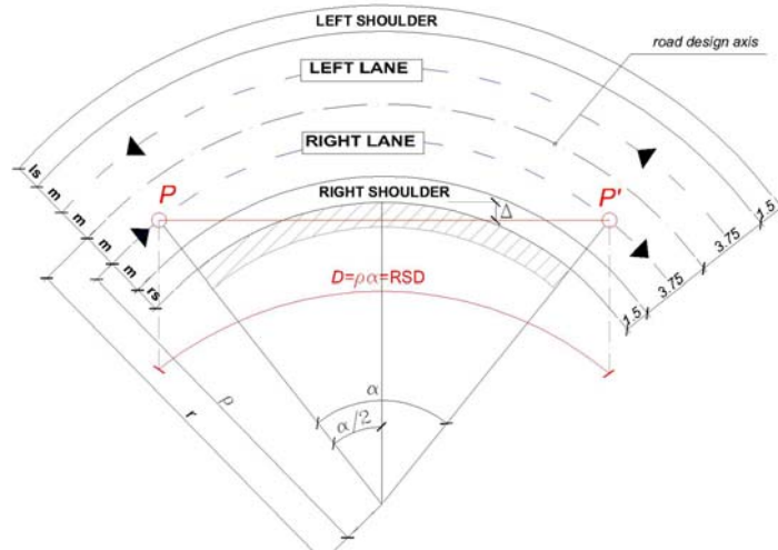
Figure 1: Cross section enlargement ( \Delta ) required in Single Carriageway right-hand bends
