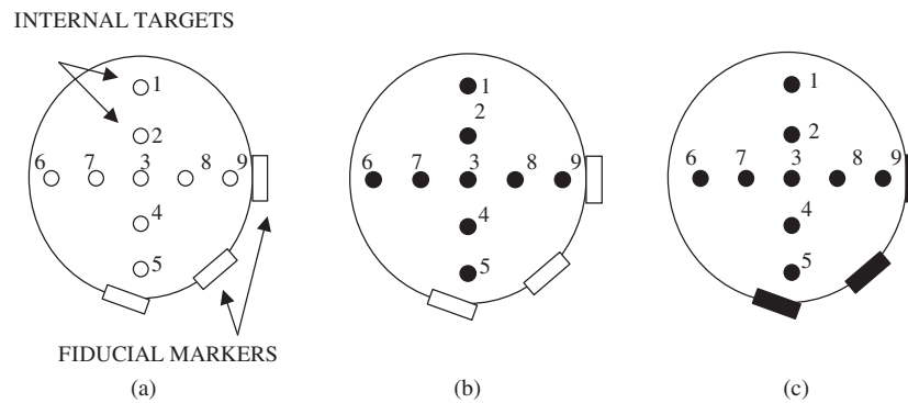
Figure 4. (a) Schematic view of the neuronavigation phantom, showing the positions of internal targets and fiducial markers. (b). In the imaging accuracy test the 1–9 internal targets are used both for the IDL registration procedure and for the accuracy evaluation. (c). In the global accuracy test the fiducial markers are used for the neuronavigator registration procedure, while the 1–9 internal targets are used for the accuracy evaluation.
