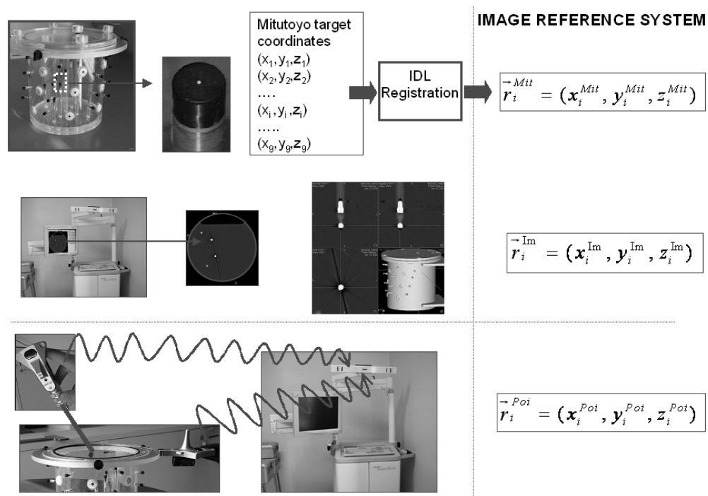
Figure 6. The three target coordinate sets: image ( \vec{r}_i^{\text{Im}} ), pointer ( \vec{r}_i^{\text{Poi}} ) and Mitutoyo ( \vec{r}_i^{\text{Mit}} ); all of them are expressed in the image reference system. Because of the high accuracy of the Mitutoyo Mechanical Touch, this coordinate set is considered as the gold standard.
