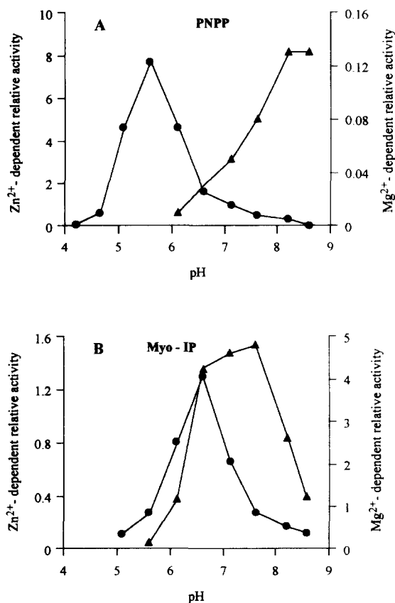
Fig. 5. pH optima of the p -nitrophenyl phosphatase (A) and myo -inositol 1-phosphatase (B) in the presence of 5 mM Zn^{2+} and 2 mM Mg^{2+} ions. The symbols are as follows: (●) Zn^{2+} -dependent, and (▲) Mg^{2+} -dependent activities. The buffers used were: pH 4.2–7.1, 25 mM sodium 3,3-dimethylglutarate; pH 7.6–8.6, 50 mM Tris-HCl. The substrate concentrations were 4 mM p -nitrophenyl phosphate, and 0.1 mM D - myo -inositol 1-phosphate.
