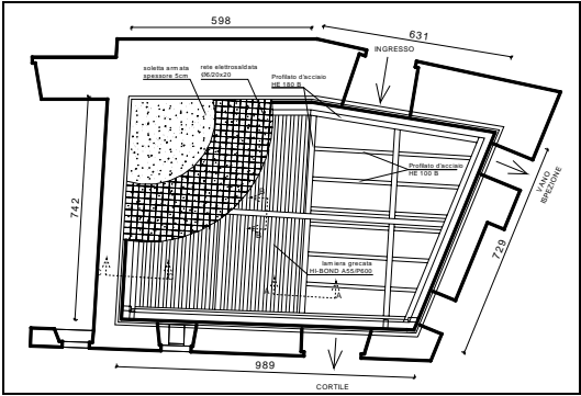
Figure 8. Structural plan of the ground floor
