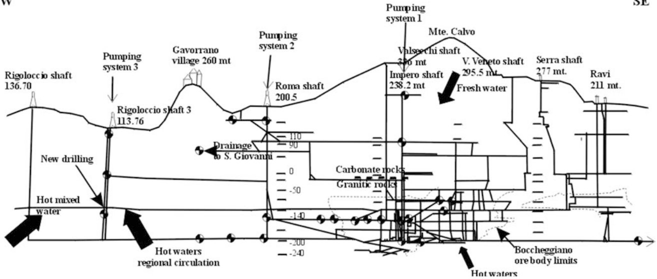
Fig. 5 Schematic section of the mine with water pumping systems and sampling points
