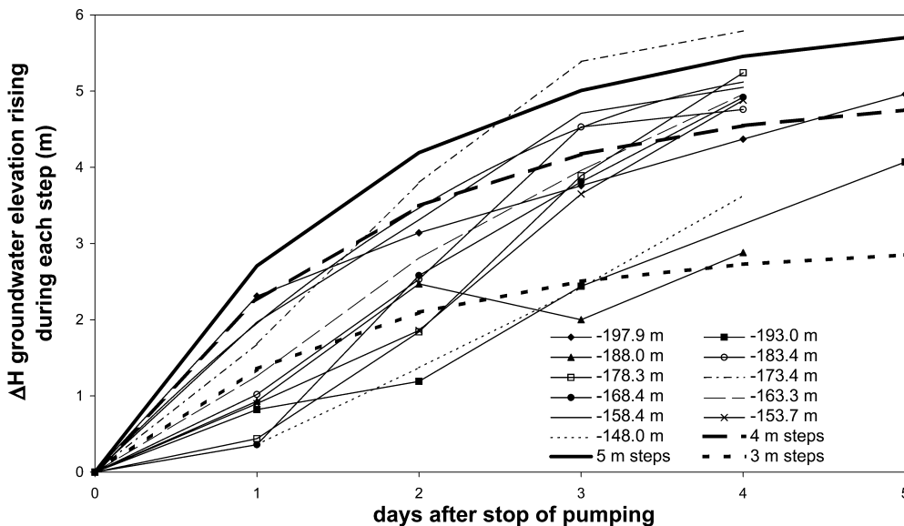
Fig. 6 Groundwater level rising during each controlled flooding step of the 1995–1999 period. Also plotted are the curves (shaded lines) calculated by using the suggested power-law function for different values of the maximum groundwater level increase
