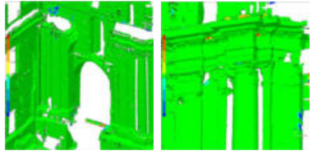
Figure 12. Comparison between the final resulting mesh and the original acquired cloud of points. As side color scale shows, green indicate deviation \leq \pm 0.005 m
