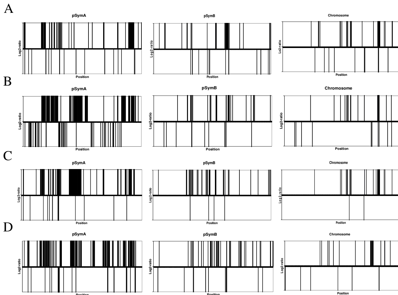
Figure 2 Location of variable ORFs along the replicons. Up and down bars indicate ORFs with Log_2\text{-ratio} > 0 (duplication) or Log_2\text{-ratio} < 0 (divergence or deletion), respectively. Thickness of bars indicates clusters of variable genes. A, AK58 strain; B, AK83 strain; C, BL225C strain; D, BO21CC strain. Replicon lengths are not in scale.
