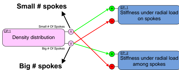
Figure 8: model of the technical contradiction: EP1 is the stiffness on spokes, EP2 is the stiffness among spokes.
