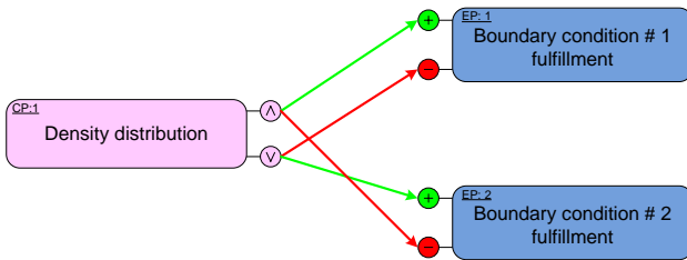
Figure 2: Geometrical contradiction derived by the comparison of two topological optimizations obtained by applying alternative boundary conditions to the technical system. It is worth to notice that The density distribution is not a scalar variable, but a 3D-array representing the optimized density of each voxel of the design space.
