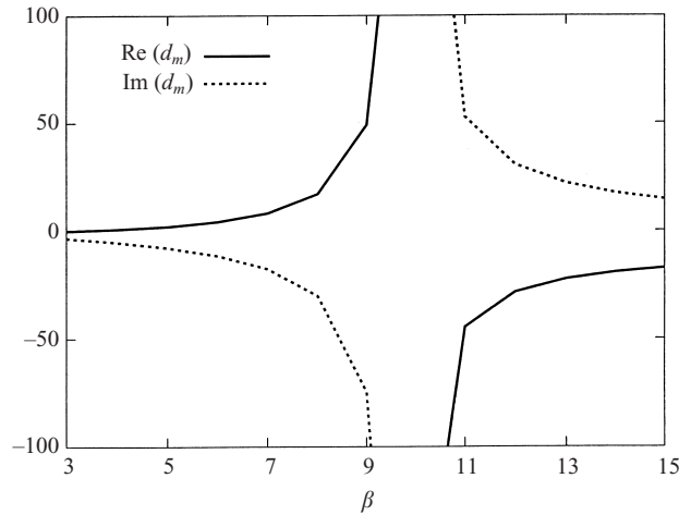
FIGURE 18. The values of topographically induced component of flow depth d_m(m = 1) is plotted versus the width ratio \beta . (Values of the relevant parameters are \theta_0 = 0.6 , \lambda = 0.09 , d_s = 2 \times 10^{-5} , R_p = 4 .) Note the occurrence of a resonant peak.
