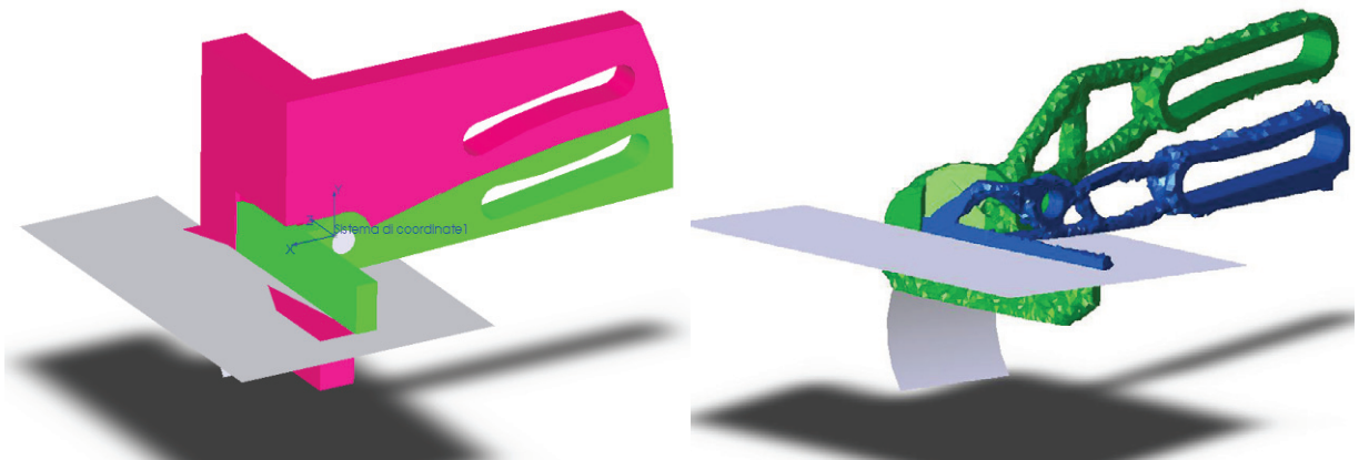
Fig. 1-Design space of a redefined optimization task (left); optimized design of a sheet metal snips (right).
