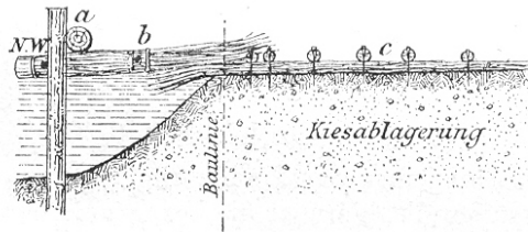
Fig. 9 – Groynes [Wang 1903]
