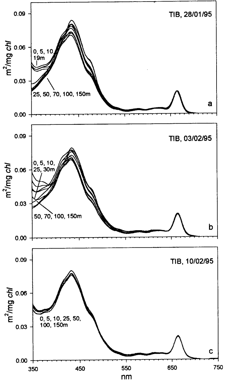
Fig. 5 - Specific absorption coefficient spectra ( m^2/mg\ chl ) of acetonetic extracts of phytoplankton at TIB from 28.01.95 to 10.02.95
