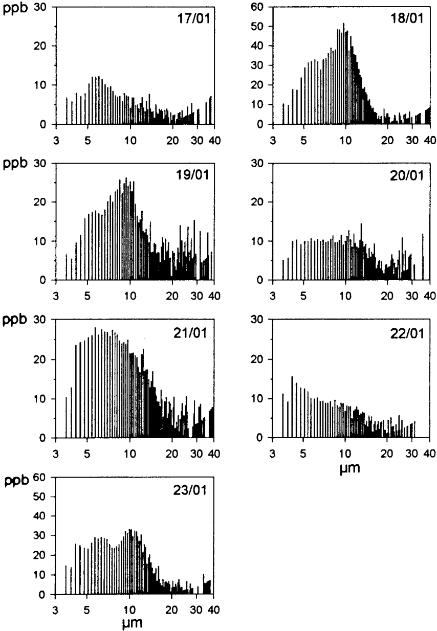
Fig. 1. Particles volume size spectra (ppb) at BTN
