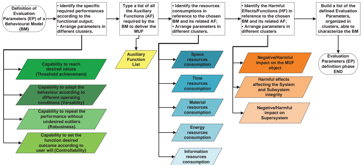
Figure 6: Algorithm for EP classification.
