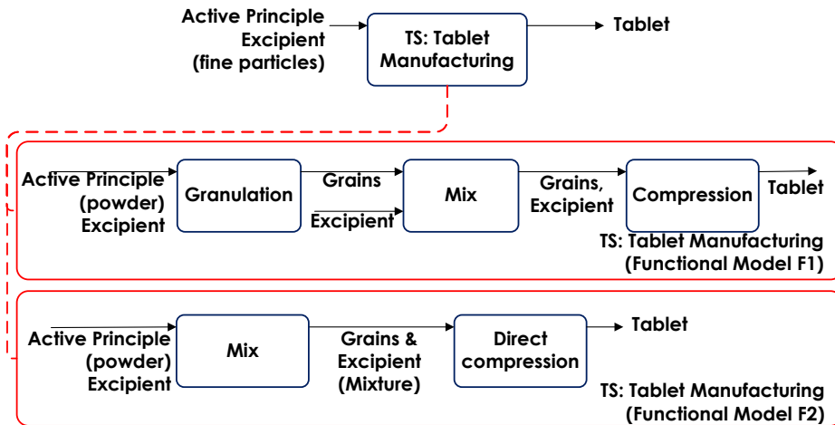
Figure 3: Functional model of a pharmaceutical tablet manufacturing process: EMS functional decomposition.
