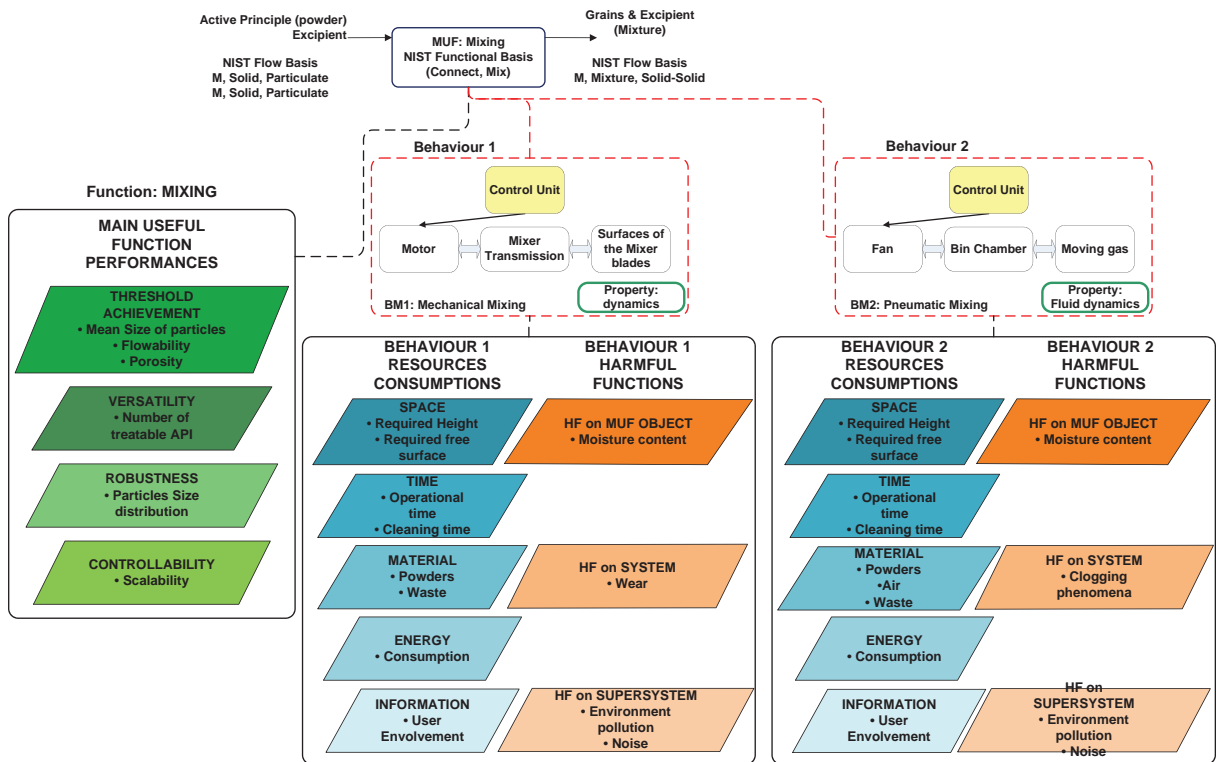
Figure 9: Exemplary EP extraction and classification for two different Behavioral Models associated to the same elementary function
