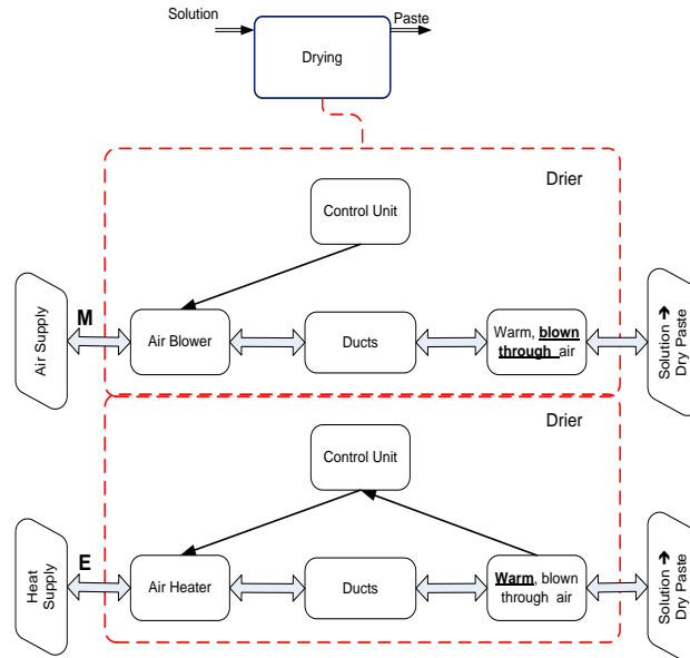
Figure 4: Exemplary Behavior represented through the model of the Minimal Technical System associated to an elementary function described through the EMS model [2].
