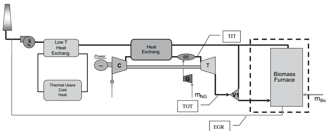
Fig. 1 – Scheme of the Bio_MGT plant.
