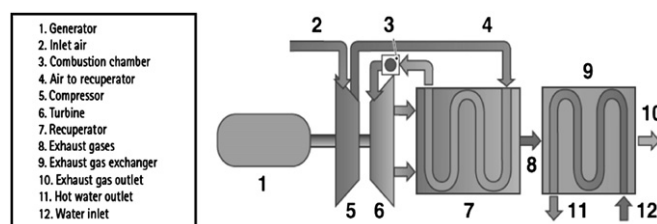
Fig. 2 – Regenerative Cycle and main component for a typical MGT (courtesy by Turbec).
