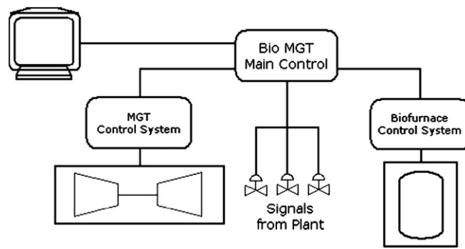
Fig. 4 – Scheme of Main Control and Monitoring system.
