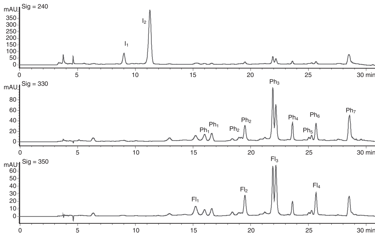
Figure 2 Chromatographic profiles at 240, 330 and 350 nm of the hydroalcoholic extract of Lippia citriodora H.B.K. I 1 , hastatoside; I 2 , verbenalin; Ph 1 , \beta -OH verbascoside; Ph 2 , \beta -OH isoverbascoside; Ph 3 , verbascoside; Ph 4 , isoverbascoside; Ph 5 , eukovoside or isomer; Ph 6 , eukovoside or isomer; Ph 7 , eukovoside or isomer; Fl 1 , luteolin-7- O -diglucuronide; Fl 2 , apigenin-7- O -diglucuronide; Fl 3 , luteolin-7- O -glucuronide; Fl 4 , apigenin-7- O -glucuronide.
