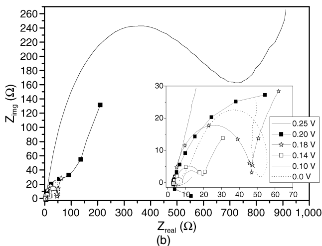
FIGURE 3. EIS spectra ([A] Bode plots, [B] Nyquist plot) obtained on Indium-WB-coated samples in artificial sweat solution at different potentials. Inset of Figure 3(b) displays a detail of the region. Potentials as described in the legend.
