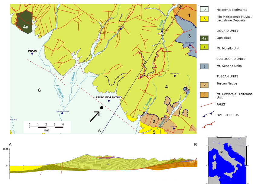
Fig. 1. Sketch map of the study area, outlining its main geological and structural features. The arrow marks the location of the measurement site. At the bottom, the geological section through points A–B in the map. The inset at the bottom right shows location of the study area with respect to Italy. The map is modified from Sheet 263 of the Geological Cartography series of the Regione Toscana, available at http://www.regione.toscana.it , last accessed December 2010.
