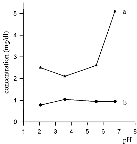
Fig. 4 Total bilirubin concentration as a function of pH for the homogenized (a) and centrifugated (b) samples obtained from the same drawn gastric content.
