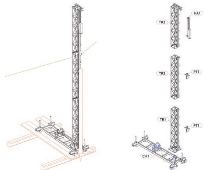
Figure 2. The pile driver on ground, and its major components.
