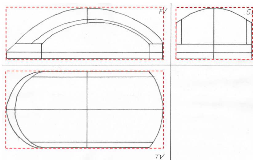
Fig. 4. Bounding boxes for the three orthographic views.
