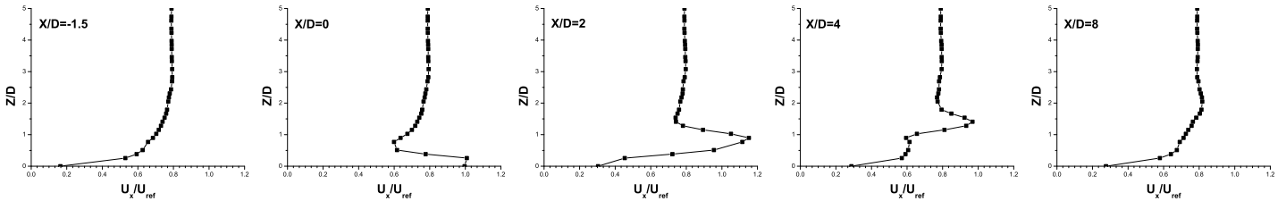
Figure 8. Mean streamwise velocity profiles for 30° case ( Ma_b = 0.1 ).
