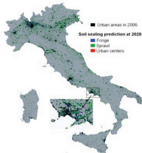
Figure 8. New soil sealing morphotypes probability: results of the multinomial model.
