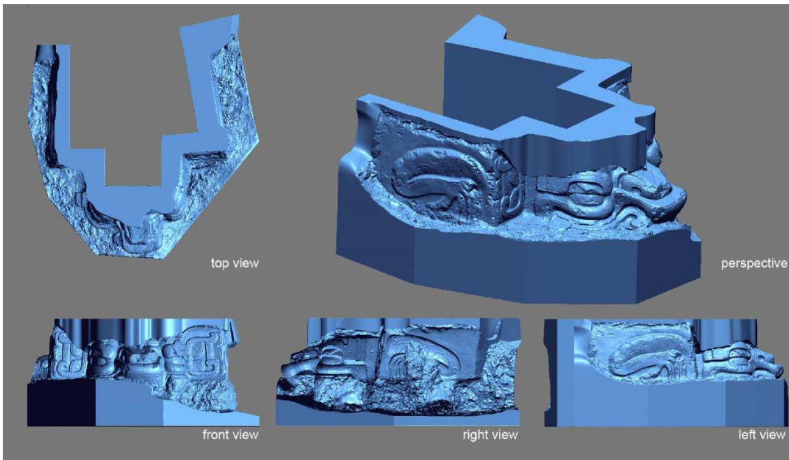
Fig. 11 – Orthographic views of the final high-poly model
