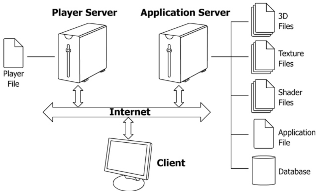
Fig. 15 – Client/Server hardware architecture of the proposed on-line 3D simulation
