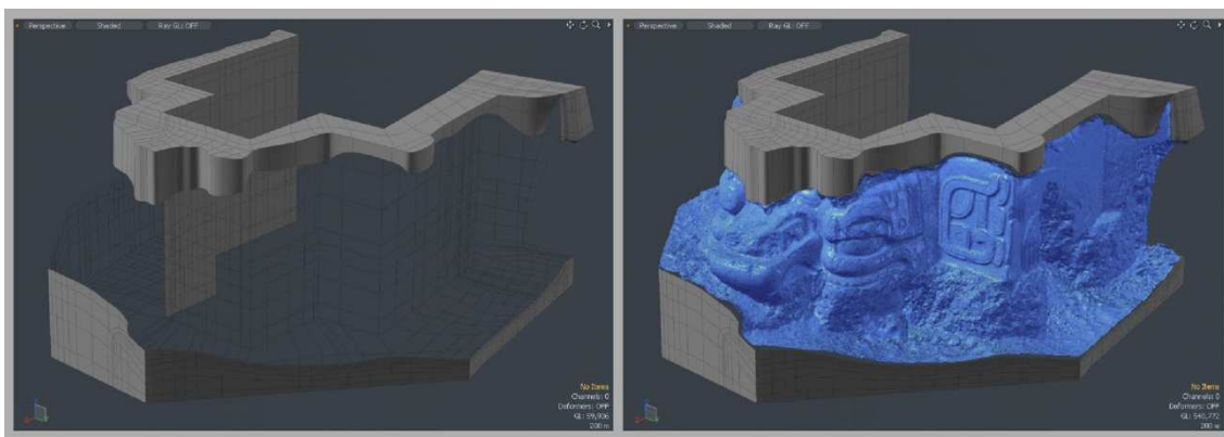
Fig. 10 – External cage created through subdivision surface modelling. It is important to notice the capability of Catmull-Clark extended to create sharp creases without having to increase the number of polygons
