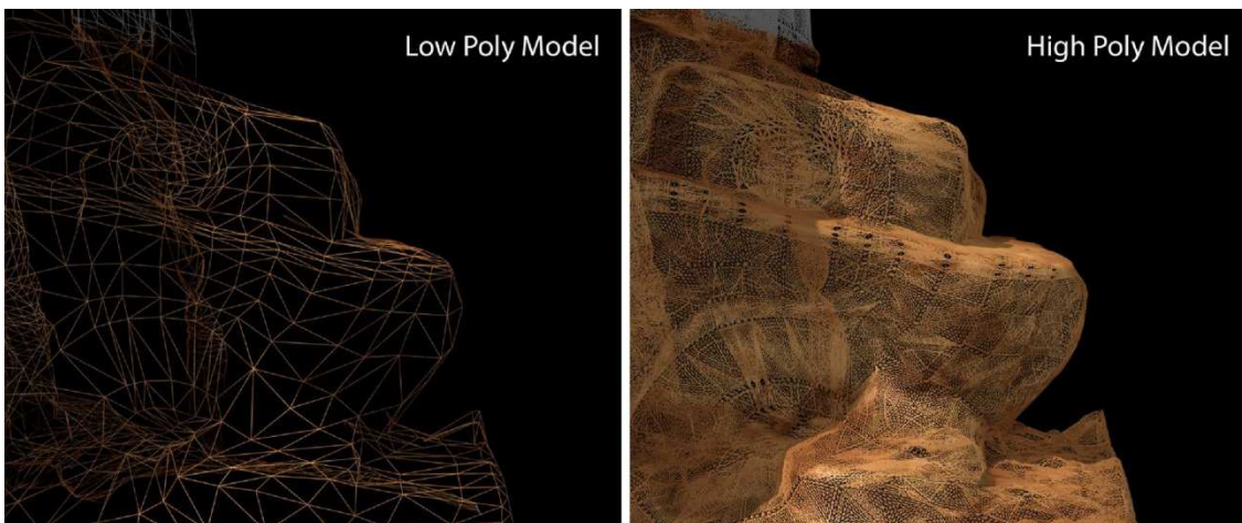
Fig. 17 – Two different Levels of Detail for geometry in the developed simulation
