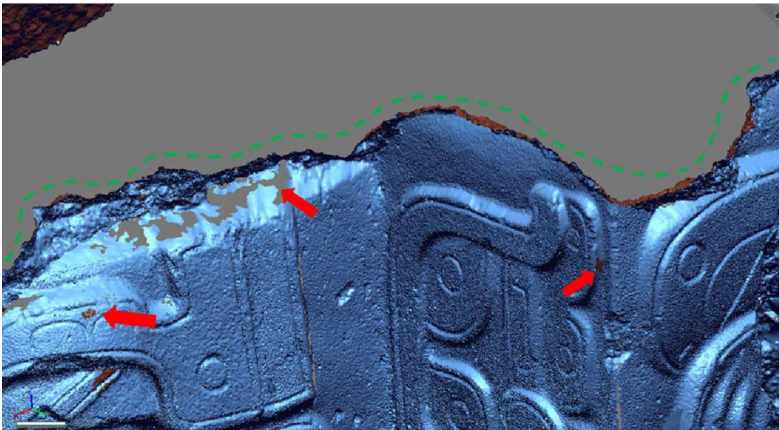
Fig. 8 – Some smaller topological problems can be easily managed inside the reverse modeling application but, the irregular hole on the top and bottom of the mascarón needs a direct modeling approach
