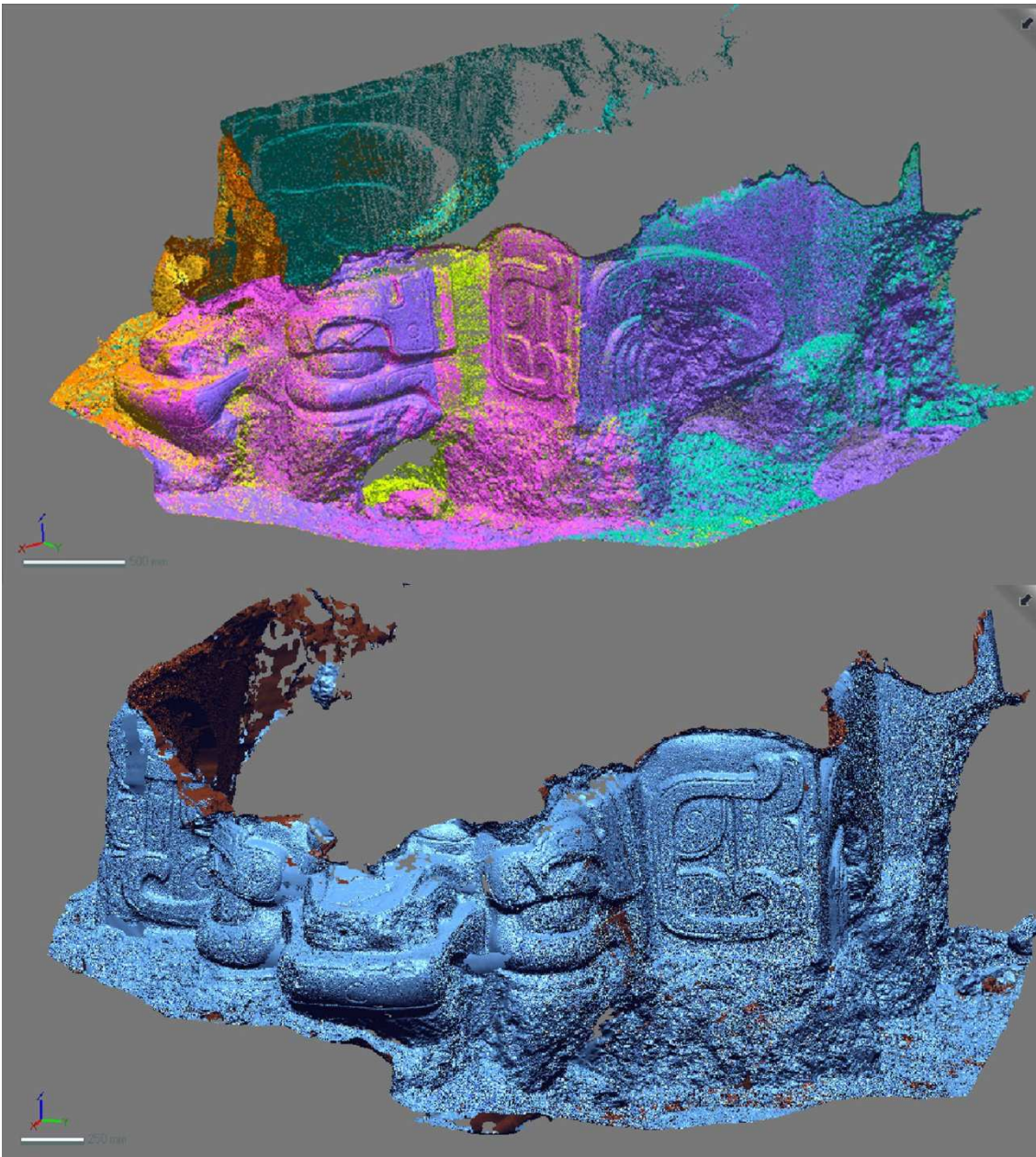
Fig. 7 – The point cloud set and the result of the meshing phase
