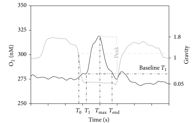
FIGURE 9: Characterisation of an oxygen burst measured with an oximeter: T_0 is the time of the onset of microgravity; T_1 is the time when the burst of oxygen begins. Its value in the Y-axis is taken as the baseline for the calculation of the area, amplitude, and duration between T_1 and T_{end} .
