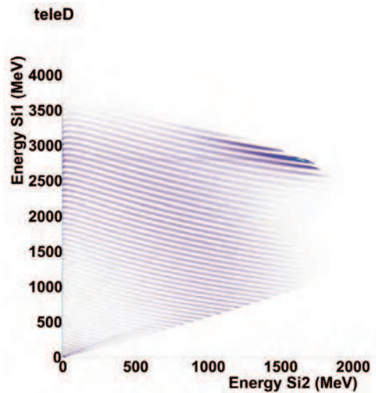
Figure 1: ΔE-E correlation for a Si(300μm) – Si (300μm), obtained with the 129 Xe beam.
