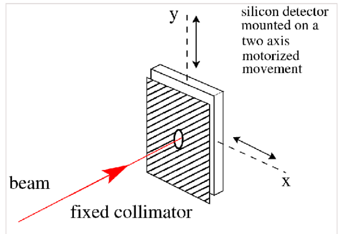
FIG. 1: Sketch of the used experimental apparatus. A remotely controlled support can move the detector along two perpendicular directions, thus allowing for an xy detector scan.
