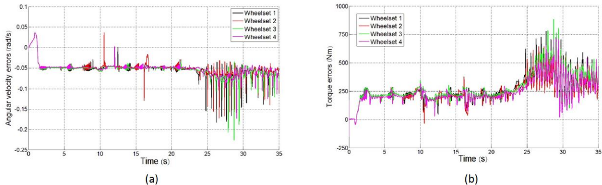
Figure 5: (a) Angular velocity error e_\omega - (b) Torque estimation error e_c
