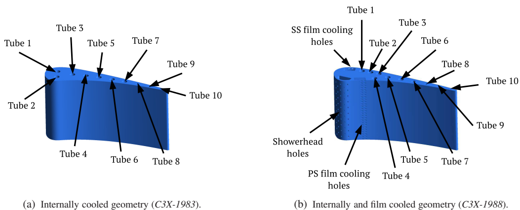
Fig. 2: Studied geometries.
