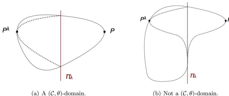
FIGURE 1. Every maximal cap of a (\mathcal{C}, \theta) -domain has Lipschitz boundary.
