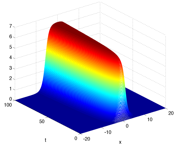
Figure 7: Dirichlet boundary conditions. Difference with the initial value for the numerical Hamiltonian and augmented Hamiltonian (left plot) when solving problem (101)-(102) with \gamma = 1 , by using HBVM(5,1) with stepsize h = 0.1 , along with the computed solution (right plot).
