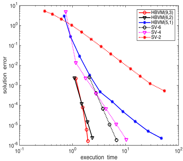
Figure 10: Work-Precision Diagram (left plot) and Hamiltonian error versus execution time (right plot) for problem (101)-(102).
