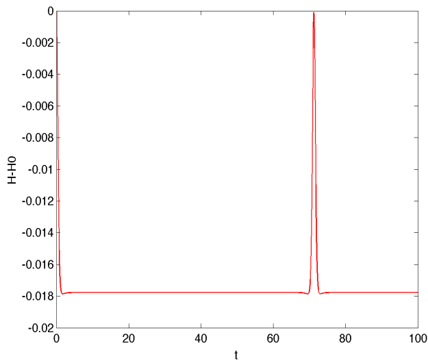
Figure 8: Neumann boundary conditions. Difference with the initial value for the numerical Hamiltonian and augmented Hamiltonian (left plot) when solving problem (101)-(102) with \gamma = 1 , by using HBVM(1,1) with stepsize h = 0.1 , along with the computed solution (right plot).
