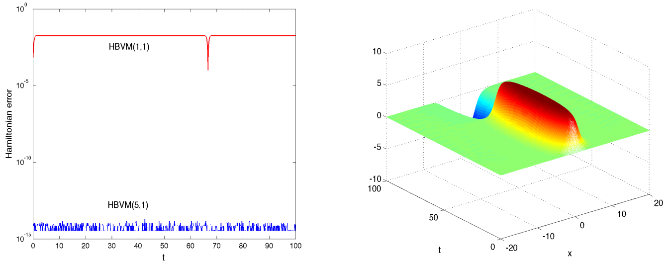
Figure 4: periodic boundary conditions and Fourier-Galerkin approximation. Hamiltonian error (left plot) when using the HBVM(1,1) and HBVM(5,1) methods with stepsize h = 0.1 , and numerical solution provided by HBVM(1,1) (right plot) when solving problem (101)-(102) with \gamma = 1 .
