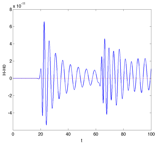
Figure 7: Dirichlet boundary conditions. Difference with the initial value for the numerical Hamiltonian and augmented Hamiltonian (left plot) when solving problem (101)-(102) with \gamma = 1 , by using HBVM(5,1) with stepsize h = 0.1 , along with the computed solution (right plot).
