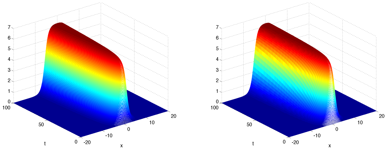
Figure 5: periodic boundary conditions. Computed solution by HBVM(5,1) with stepsize h = 0.1 by using a finite-difference spatial discretization (left plot) or a spectral space discretization (right plot).
