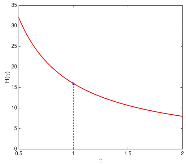
Figure 2: Double-pole solution for \gamma = 1 (left plot), and Hamiltonian as a function of \gamma (right plot).
