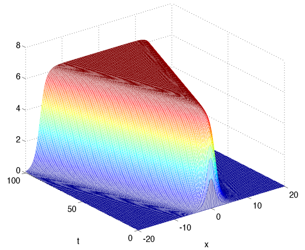
Figure 1: Breather solution for \gamma = 1.01 (left plot), and kink-antikink solution for \gamma = 0.99 (right plot).
