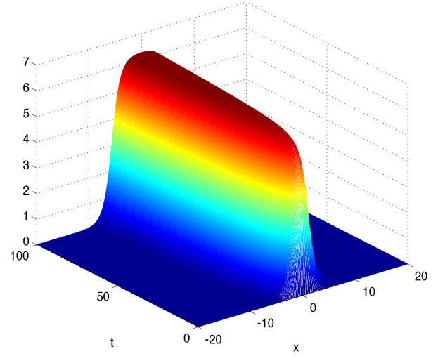
Figure 9: Neumann boundary conditions. Difference with the initial value for the numerical Hamiltonian and augmented Hamiltonian (left plot) when solving problem (101)-(102) with \gamma = 1 , by using HBVM(5,1) with stepsize h = 0.1 , along with the computed solution (right plot).
