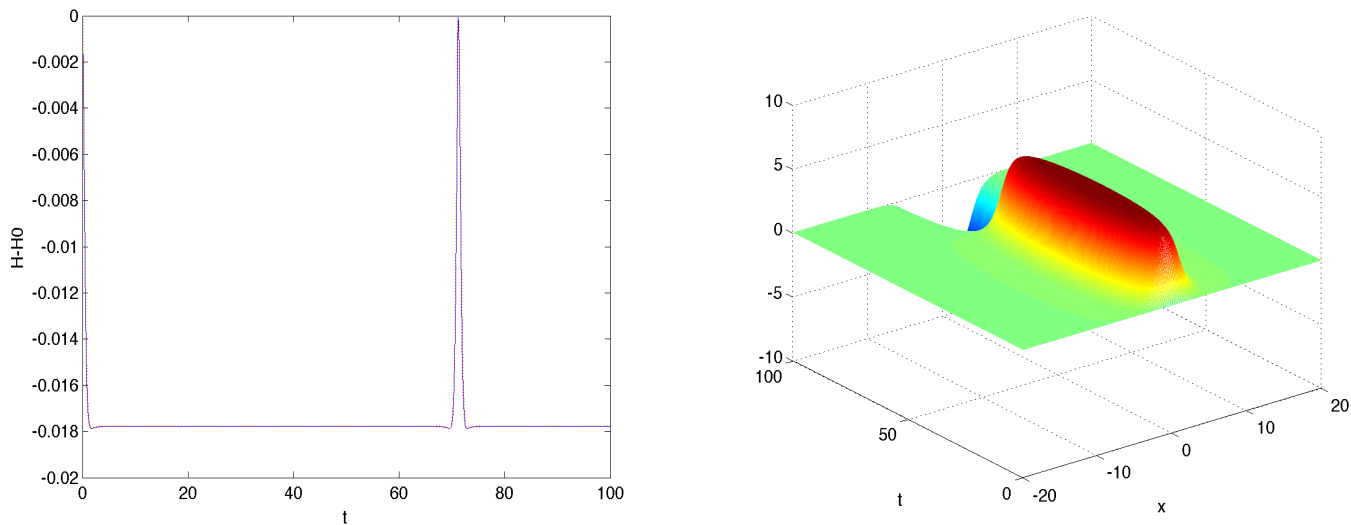
Figure 6: Dirichlet boundary conditions. Difference with the initial value for the numerical Hamiltonian and augmented Hamiltonian (left plot) when solving problem (101)-(102) with \gamma = 1 , by using HBVM(1,1) with stepsize h = 0.1 , along with the computed solution (right plot).
