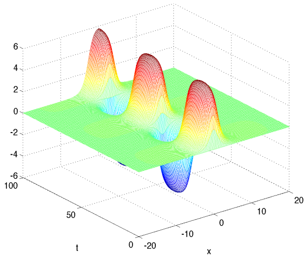
Figure 1: Breather solution for \gamma = 1.01 (left plot), and kink-antikink solution for \gamma = 0.99 (right plot).
