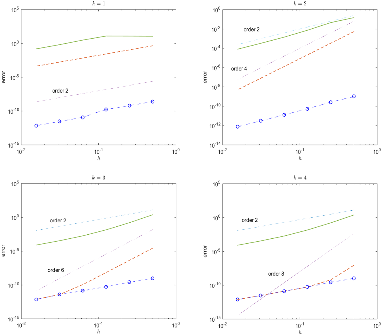
Figure 11: Sine-Gordon problem (101)-(102) with \gamma = 1 , Dirichlet boundary conditions and finite-difference semi-discretization with N = 400 , solved by means of HBVM( k, 1 ), k = 1, 2, 3, 4 . Errors at time t = 100 versus time-step for the solution (solid line), the Hamiltonian function H (dashed line) and \tilde{p} (dotted line with circles).
