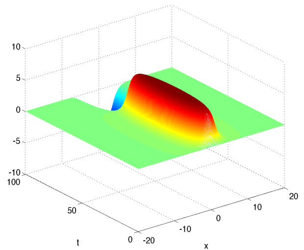
Figure 8: Neumann boundary conditions. Difference with the initial value for the numerical Hamiltonian and augmented Hamiltonian (left plot) when solving problem (101)-(102) with \gamma = 1 , by using HBVM(1,1) with stepsize h = 0.1 , along with the computed solution (right plot).
