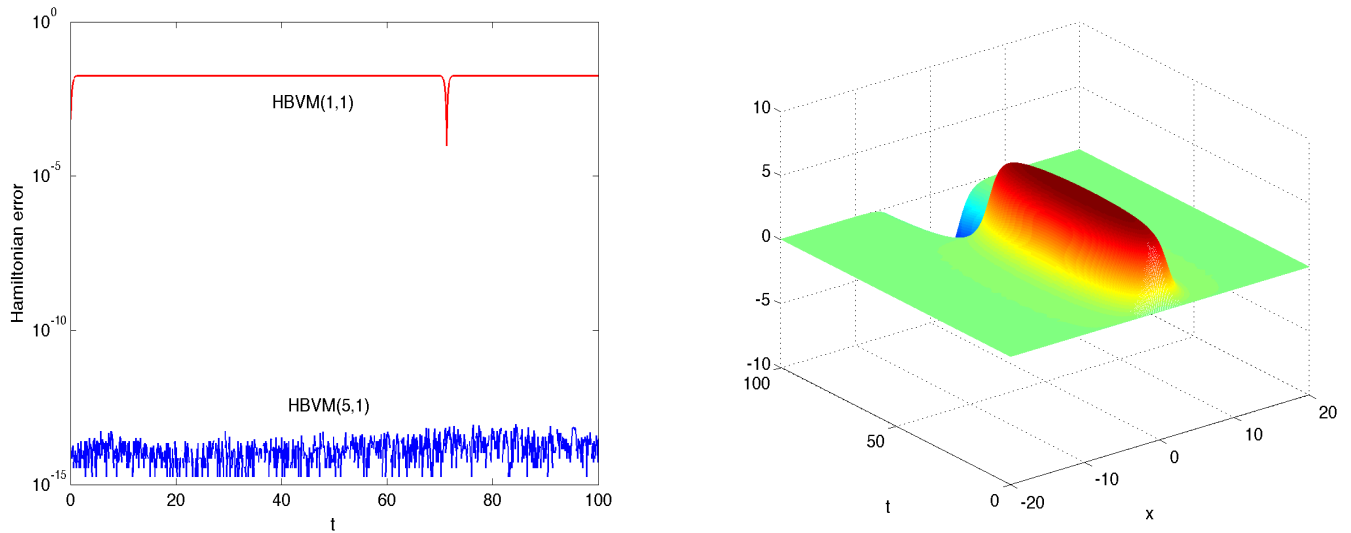
Figure 3: periodic boundary conditions and finite-difference approximation. Hamiltonian error (left plot) when using the HBVM(1,1) and HBVM(5,1) methods with stepsize h = 0.1 , and numerical solution provided by HBVM(1,1) (right plot) when solving problem (101)-(102) with \gamma = 1 .
