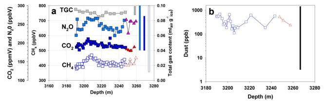
Figure 3. Gas and dust properties of the clean (squares) and dispersed (triangles) basal ice facies at EPICA Dome C: (a) total gas content ( \text{mL}_{\text{air}}\text{ice}^{-1} , grey), methane (ppbV, white), nitrous oxide (ppbV, light blue) and carbon dioxide (ppmV, dark blue) – vertical bars of equivalent shading cover the full concentration range observed for \text{CH}_4 , \text{CO}_2 , \text{N}_2\text{O} and total gas content during the preceding climatic cycles, (b) dust concentrations (ppb) – the black vertical bar covers the full concentration range during the previous climatic cycles.
