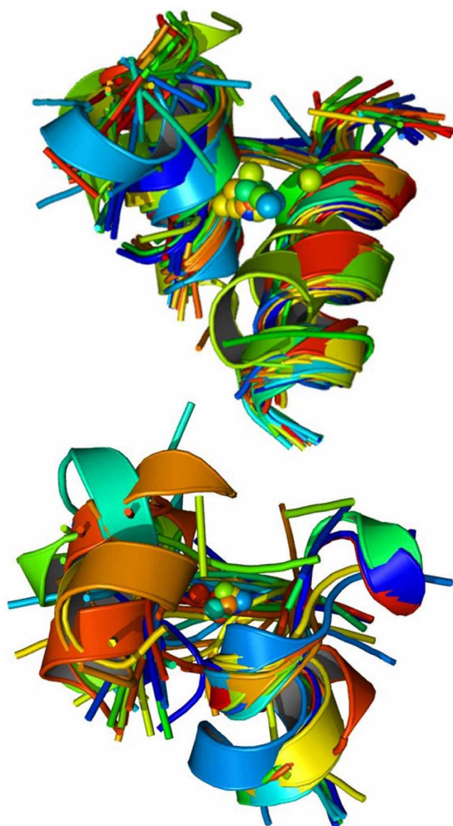
Figure 4 | Example clusters of representative zMFSs. (A) superposition of 66 representative zMFSs of different related metallopeptidases; the common position for substrate binding, as indicated by the binding of ligands (hidden for clarity) in the 3D structures of the cluster, faces the reader; (B) superposition of 31 representative zMFSs of non-standard zinc fingers.
