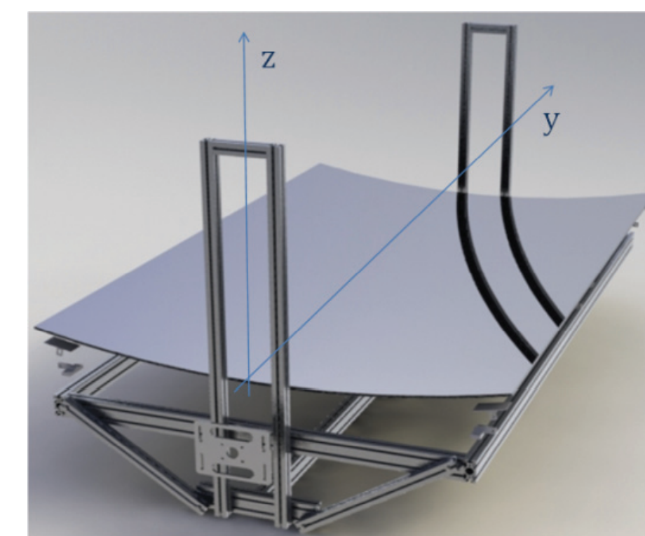
Fig. 2: Collector shaded model
