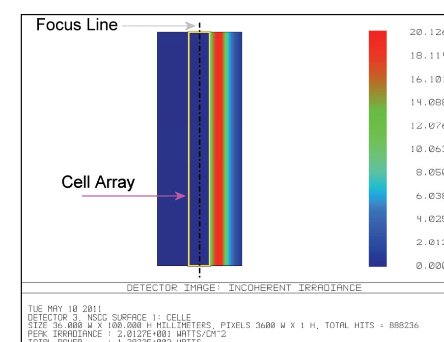
Fig. 4: Image on a detector placed in the focal plane for \delta_y=0.5^\circ . The rays fall far away from the cells zone.
