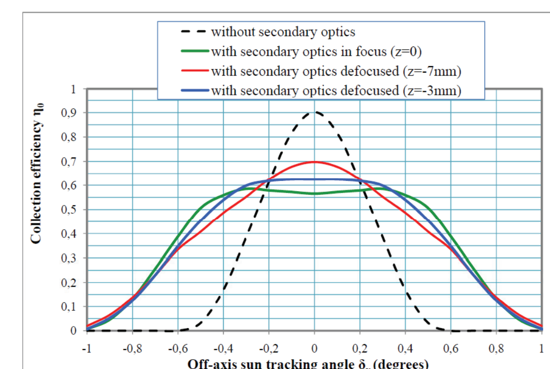
Fig. 6: Collection efficiency for different positions of secondary, vs tracking misalignment angle \delta_y .
