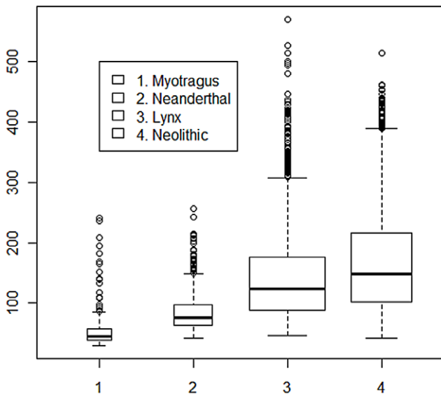
Figure 1. Sequence length distribution of the human contaminant sequences obtained from DNA extracted from bone samples of a Myotragus balearicus and an ancient lynx, and the putatively endogenous sequences from a Neolithic human and a Neanderthal specimen obtained by 454-FLX pyrosequencing. The contaminant reads in Myotragus are possibly fragmented by the bleach treatment; nevertheless, a large overlapping in the distribution length can be observed among samples. doi:10.1371/journal.pone.0024161.g001
