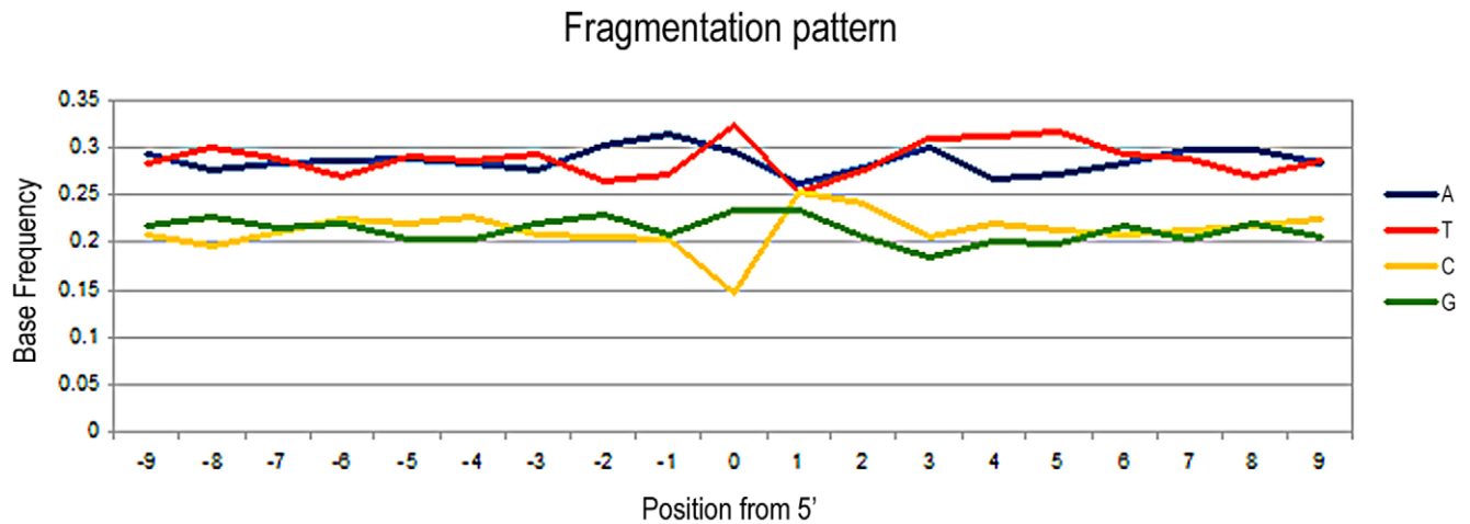
Figure 5. Nucleotide base frequencies at the 5' end of the human Neolithic sequences. The base composition is plotted as a function of distance from the 5'-end. The depurination-based pattern can be seen, despite the small sample size (N = 1,117 reads). doi:10.1371/journal.pone.0024161.g005
