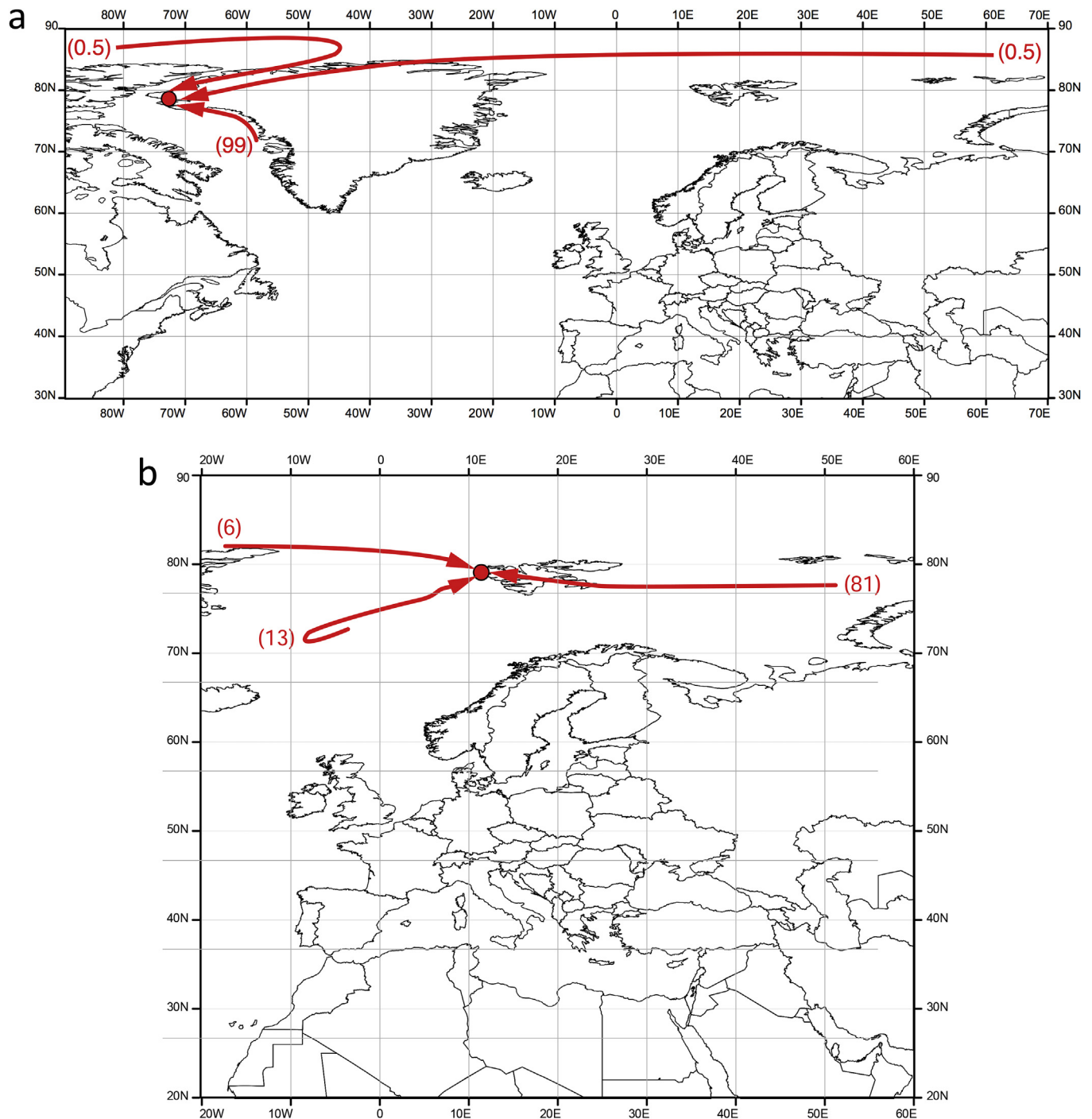
Fig. 2. Air masses origin as indicated by a cluster analysis of the 4-day backtrajectories at 200 m arriving at Thule (a) and Ny Ålesund (b) for spring-summer of years 2010–2012.
