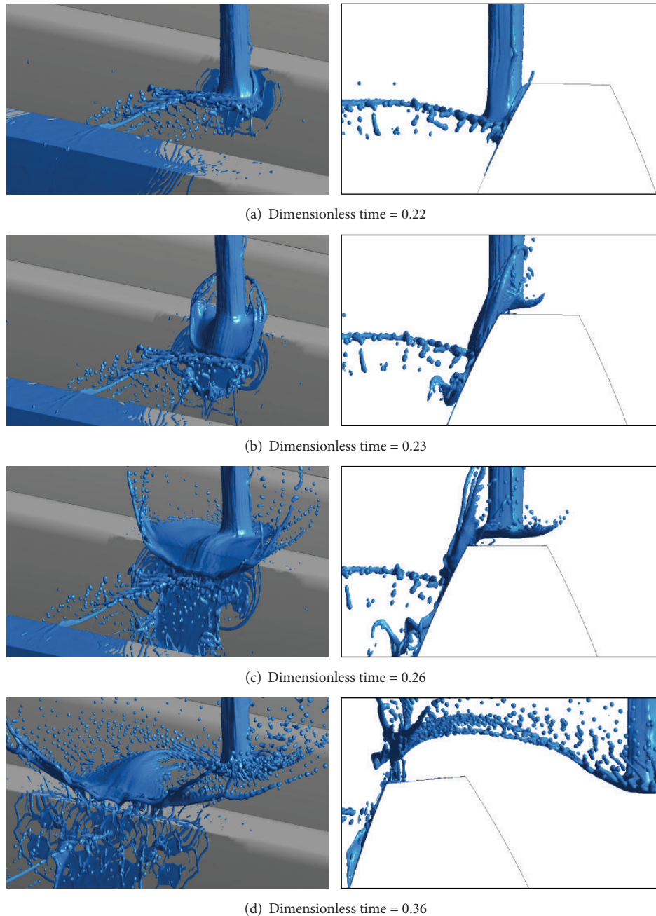
FIGURE 19: Run 3D-2: isosurface of oil volume fraction = 0.1.
