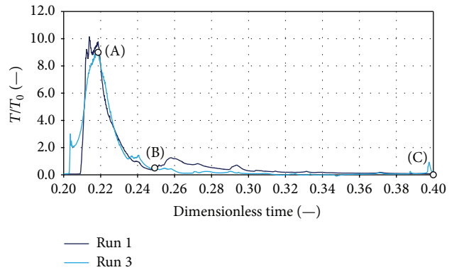
FIGURE 12: Dimensionless resistant torques during the second impact: run 1 versus run 3.
