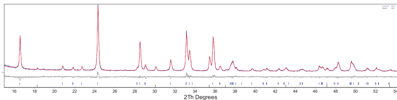
Figure 2. Rietveld refinement of the Fe08 sample pattern. The experimental pattern (blue) is compared with the calculated one (red). The difference plot (gray) and the bars at the expected angular positions of the different phases (orthosilicate s.g. P2 1 /n and magnetite) are also reported.
