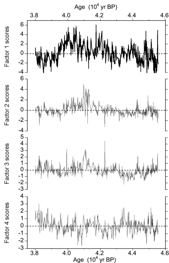
Figure 2. Temporal trend of Factor scores for Factors 1–4 produced by PCA.
