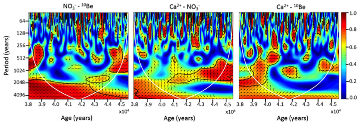
Figure 3. Wavelet coherence for nitrate and ^{10}\text{Be} (a), nitrate and calcium (b) and ^{10}\text{Be} and calcium (c) flux measured along the EDC core during the 38–45.5 kyr BP period. The colors indicate the coherence value (see the colorbar), the arrows point to the relative phase between the series (right-pointing arrows correspond to 0 degrees, up-pointing arrows –90 degrees, etc.). The areas of the 5% significance are bounded with black contours. The cone of influence, i.e., the areas of the edge effect, is shown with white lines.
