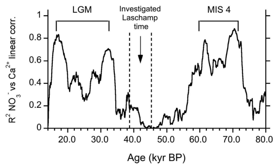
Figure 4. R^2 of the running linear correlation (5-kyr window) between nitrate and calcium flux in the last glacial period (20–80 kyr BP).
