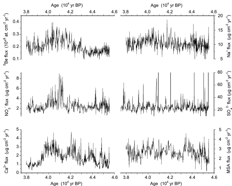
Figure 1. Flux temporal profiles for ^{10}\text{Be} and the most relevant chemical markers measured along the EDC ice core in the 38–45.5 kyr BP time period.
