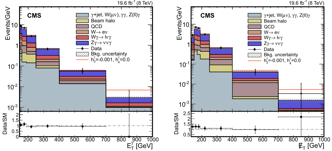
Fig. 2. The E_T^\gamma and E_T^{\text{miss}} distributions in data (points with error bars) compared with the SM Z\gamma \rightarrow \nu\bar{\nu}\gamma signal and estimated contributions from backgrounds. A typical aTGC signal from Z\gamma\gamma with h_3^\gamma = -0.001 , h_4^\gamma = 0.0 would provide an excess, as shown in the dot-dashed histogram. The background uncertainty includes statistical and systematic components.
