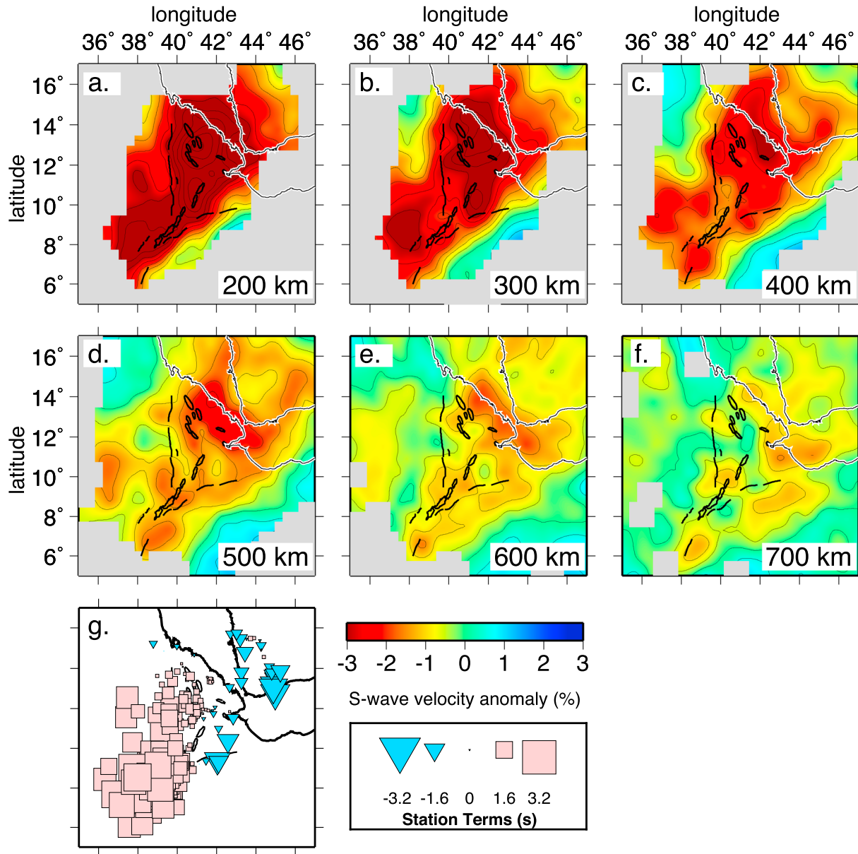
Figure 4. Depth slices through our S - SKS preferred intermediate-damped tomographic model (flattening = 4800, smoothing = 153,600, damping = 35), at depths between 200 and 700 km. Regions with less than five rays per node are shaded gray (a version where regions with less than 10 rays per node are shaded can be found in Figure S2). The spacing between the contours is 0.5%. The black lines delineate the major border faults and magmatic zones bounding the Afar Depression, and the black over white lines show the coastlines. The triangular and square symbols in Figure 4g represent the sign and magnitude of the station static terms. Compare with Figure S5 to see the first-order similarities in structure between the independently inverted S / SKS and P velocity models. Compared to the undamped model (Figure S3), the shallow mantle anomalies are enhanced and more extensive. Otherwise, similar features, including the low velocities below Afar and west of the MER, appear.
