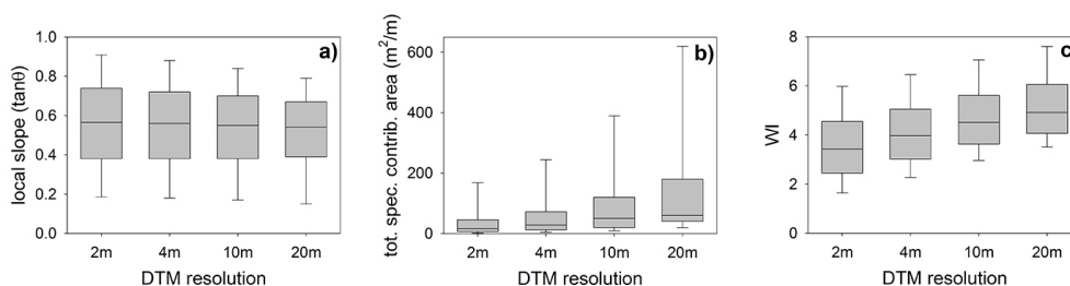
Figure 4. Box plots of topographic attributes for the four different DTM resolutions: (a) local slope, (b) total specific contributing area, (c) WI. The boxes show the 25th and 75th percentile, the whiskers show the 10th and 90th percentile, the horizontal line within the box indicates the median.
