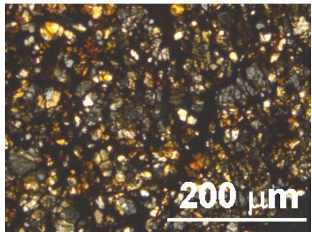
Figure 1: polarizing optical microscope image of a thin section of the enstatite chondrite NWA 7766. Cream-grey areas are enstatite, black areas are metal and troilite; transmitted light, crossed polars.
