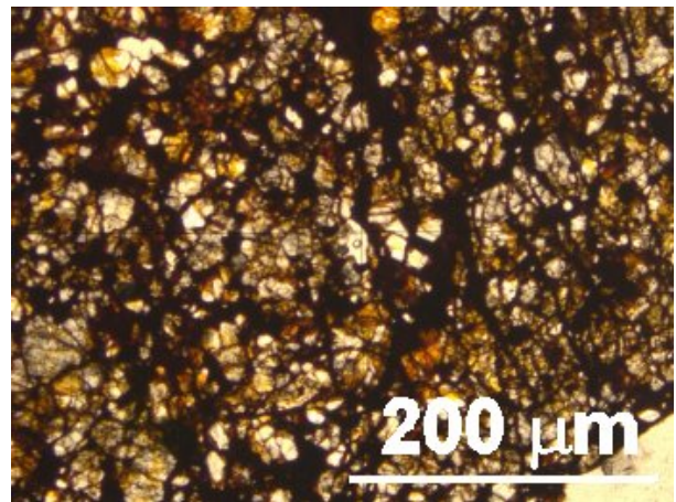
Figure 2: polarizing optical microscope image of a thin section of the enstatite chondrite NWA 7766. Yellow-creamy areas are enstatite, dark brown to black areas are metal and troilite; transmitted light, plane polars.
