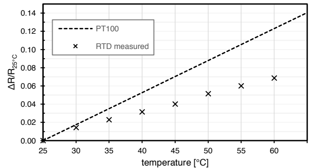
Fig. 5. Relative resistance change measured between 25°C and 60°C. The characteristic plot of a standard PT100 is shown for comparison.
