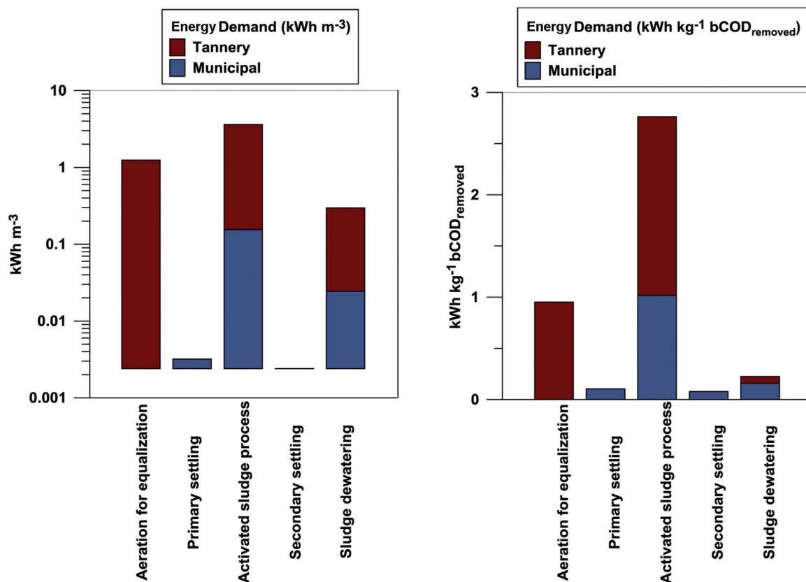
Fig. 6. Comparison of the energy demand of the tannery and municipal wastewater treatment in Italy.
